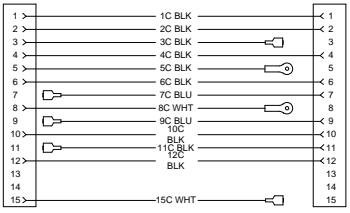
Computer harness
